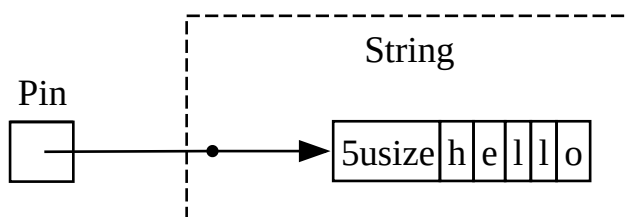
Figure 17-8: Pinning a String , with a dotted line indicating that the String implements the Unpin trait, so it is not pinned.
